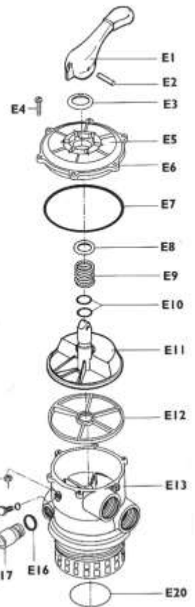
Top Mount Multiport Valve
